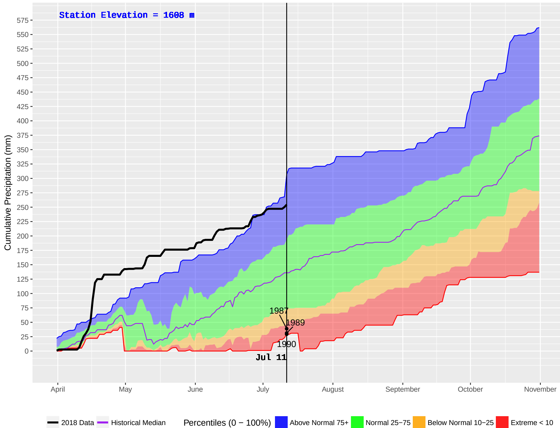
DEWAR CREEK (421) : Historical (1986–2016) and Current (2018) Noon Cumulative Precipitation
