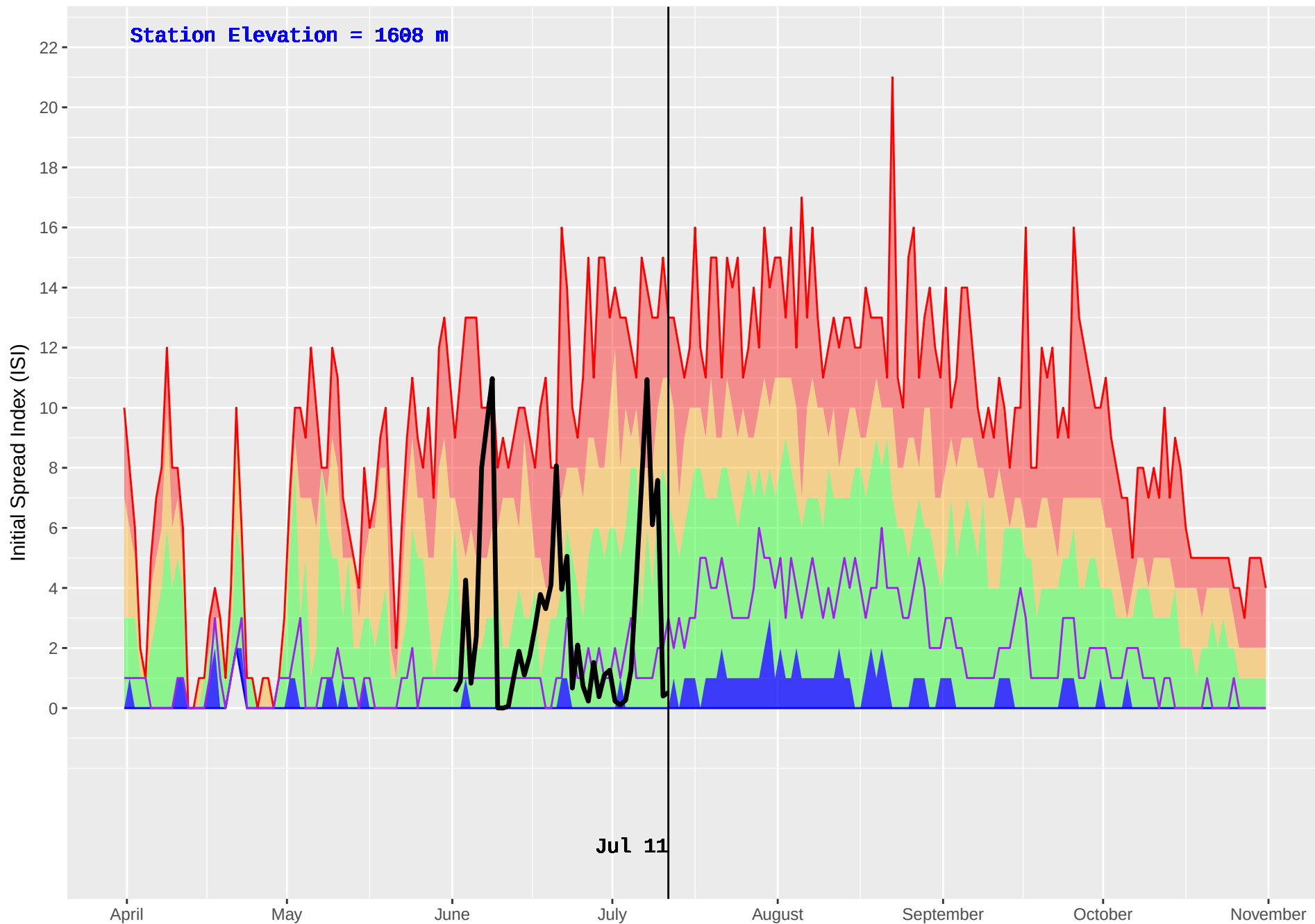
DEWAR CREEK (421) : Historical (1986–2016) and Current (2018) Noon Initial Spread Index (ISI)
