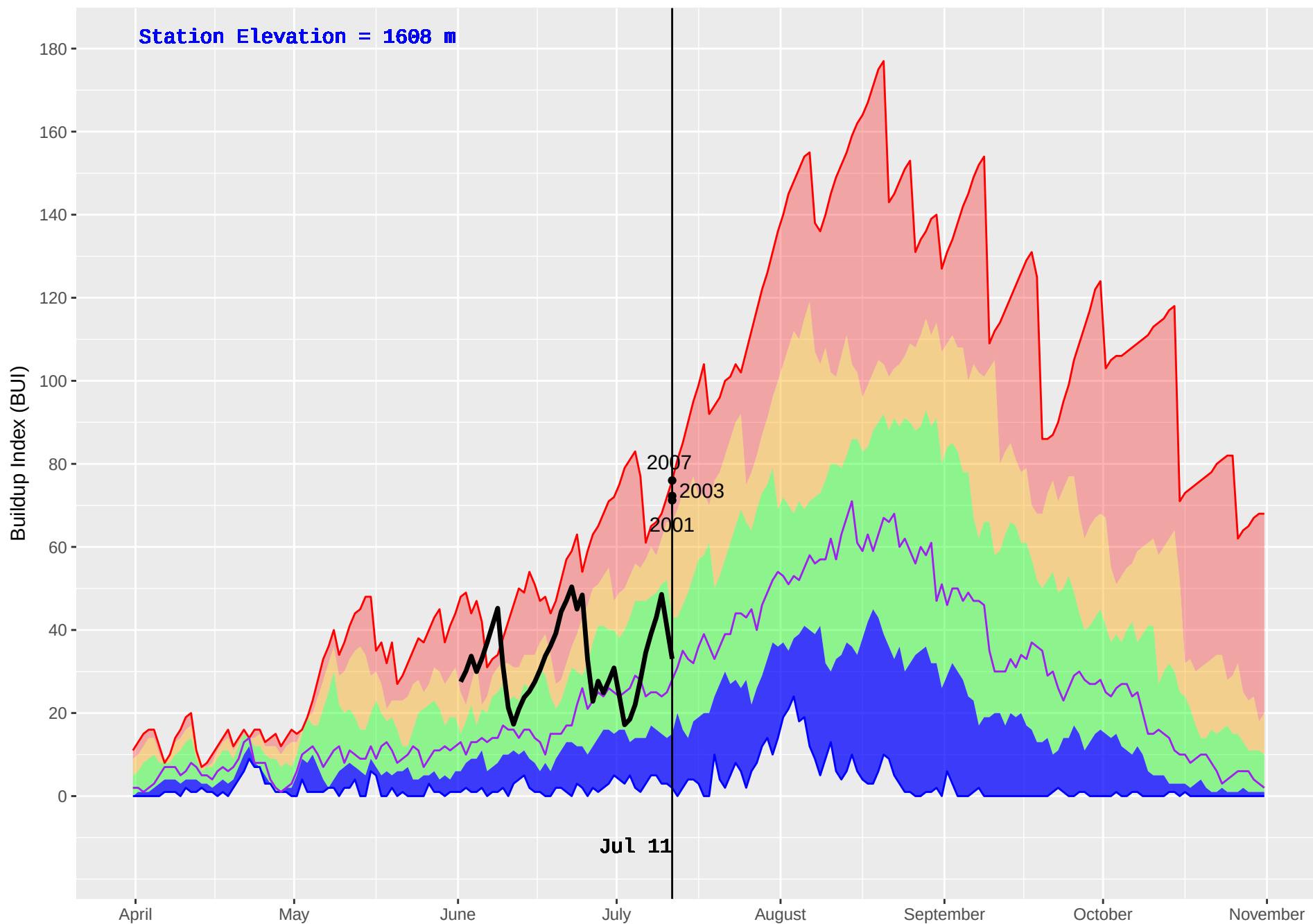
DEWAR CREEK (421) : Historical (1986–2016) and Current (2018) Noon Buildup Index (BUI)
